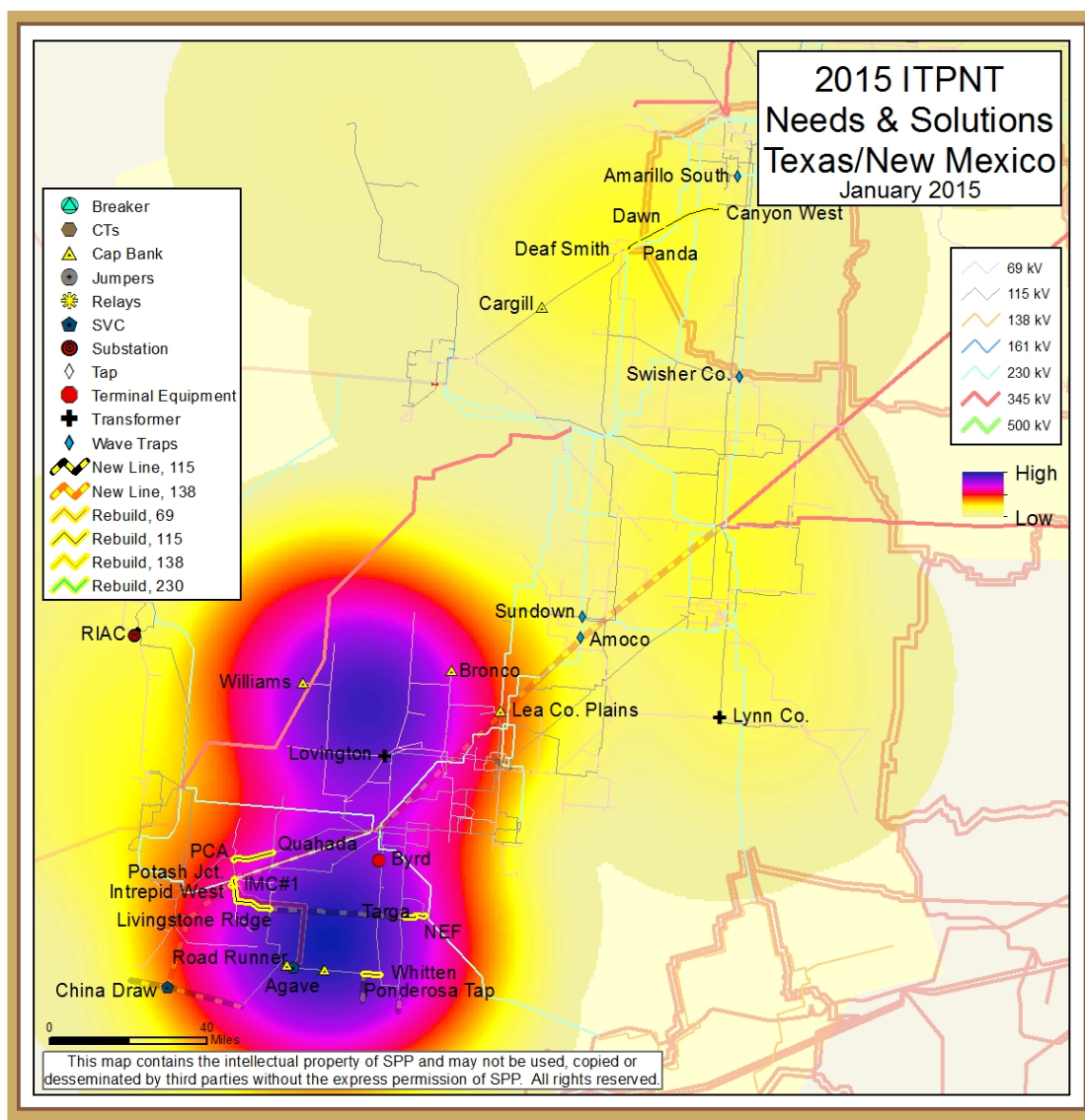
Figure 5.8: 2015 ITPNT West Texas & New Mexico Area Solutions
