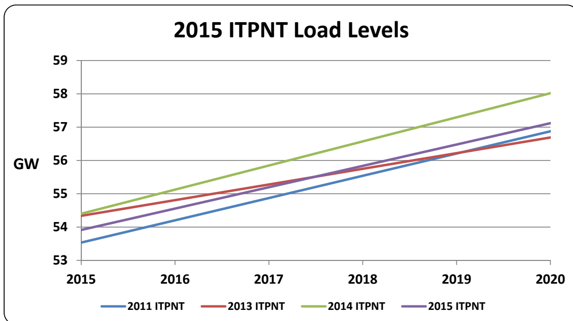
Figure 3.2: ITPNT Load Levels Comparisons
