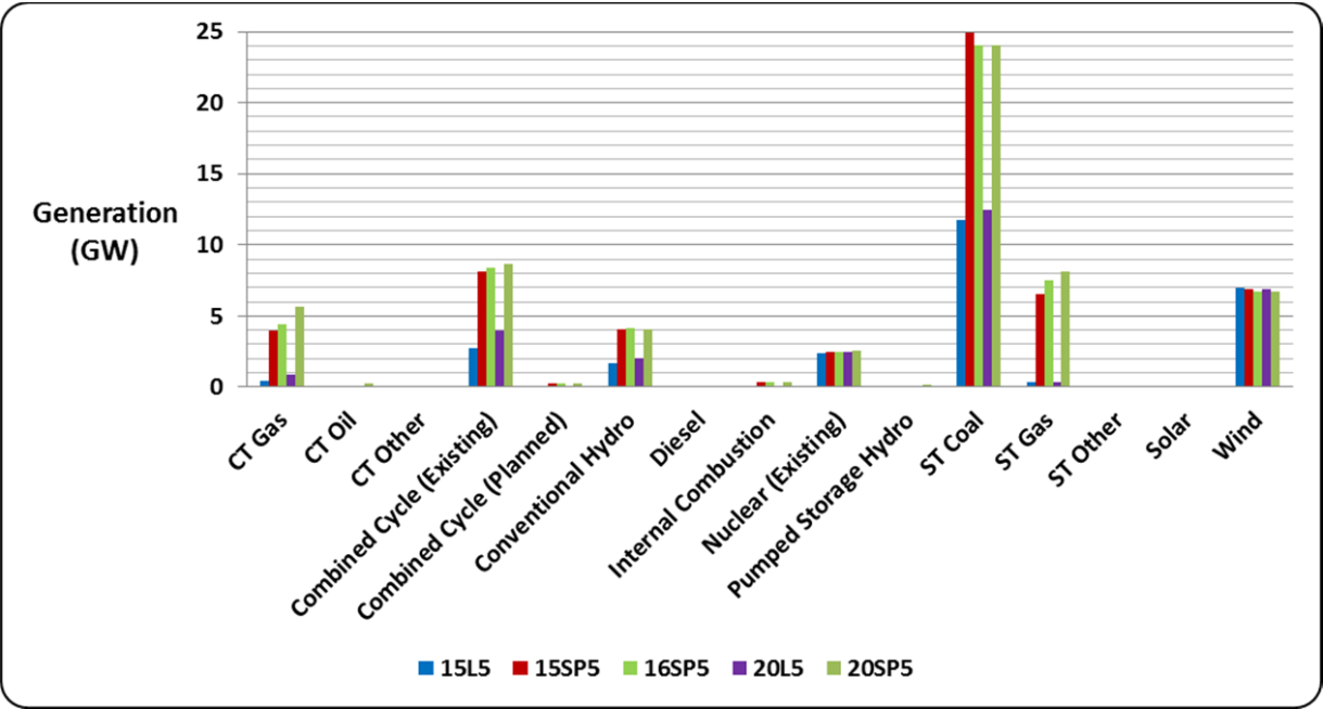
Figure 3.4: 2015 ITPNT Generation Mix Scenario 5
