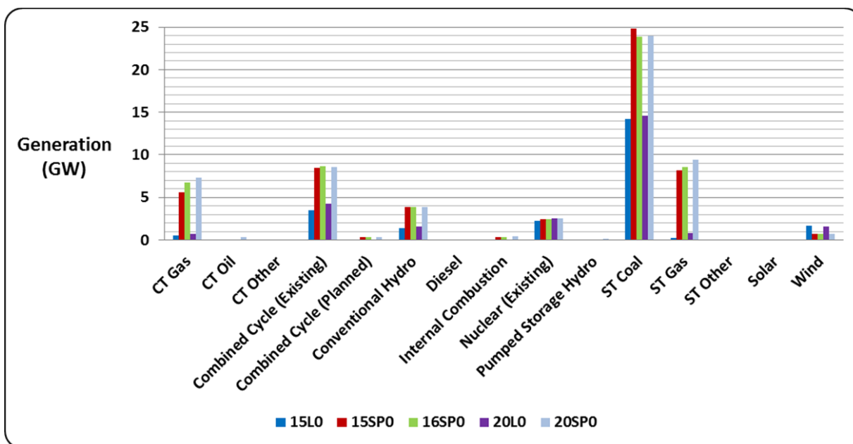
Figure 3.3: 2015 ITPNT Generation Mix Scenario 0
