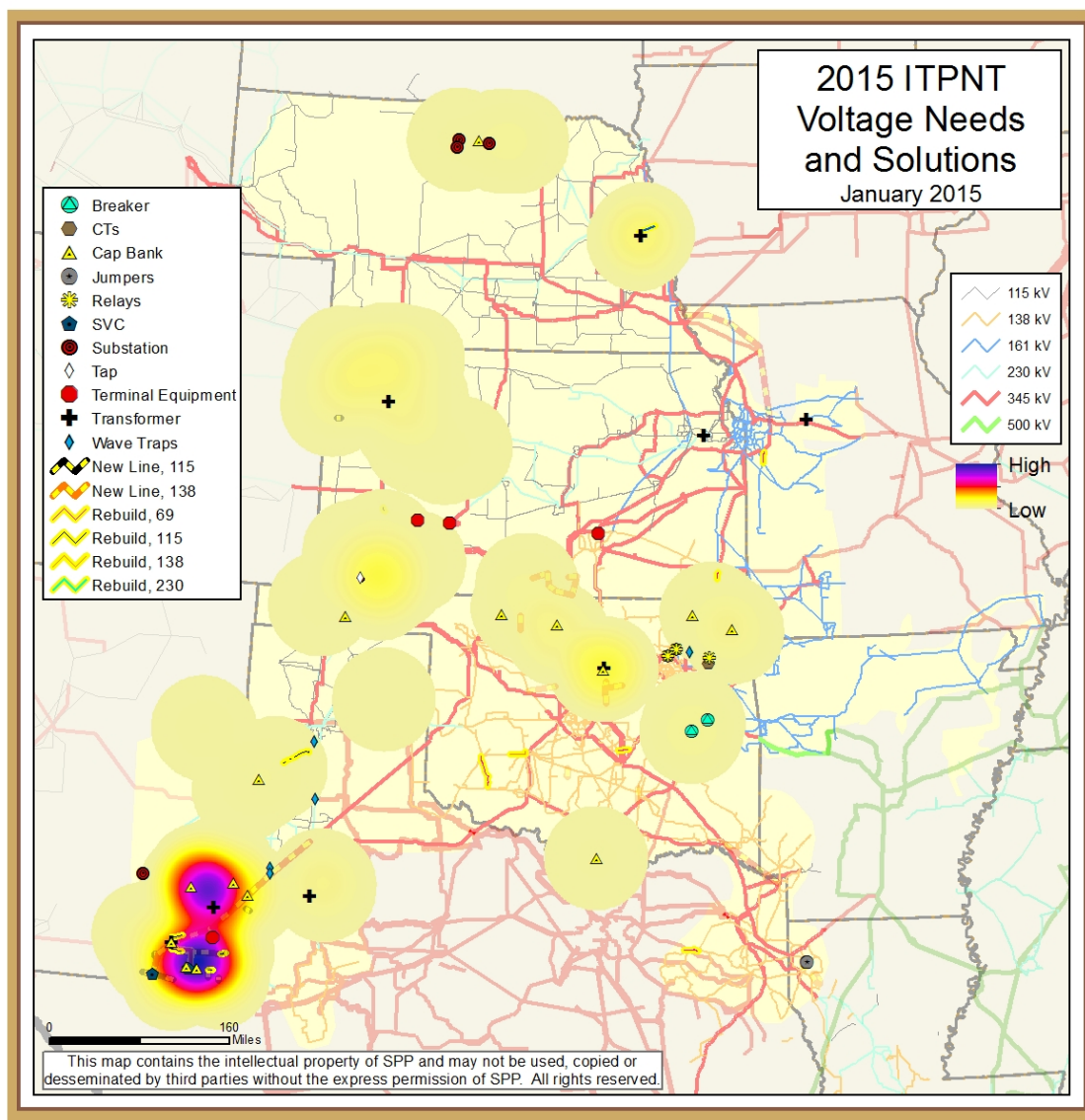
Figure 0.2: 2015 ITPNT Voltage Needs and Solutions
