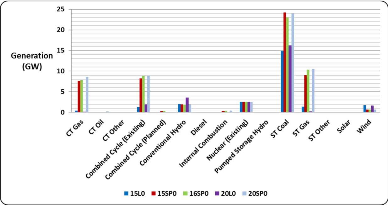
Figure 3.5: 2015 ITPNT CBA Generation Mix
