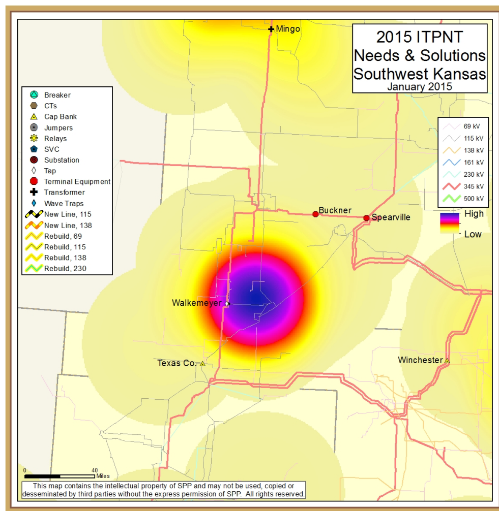
Figure 5.9: 2015 ITPNT West Kansas Solutions
