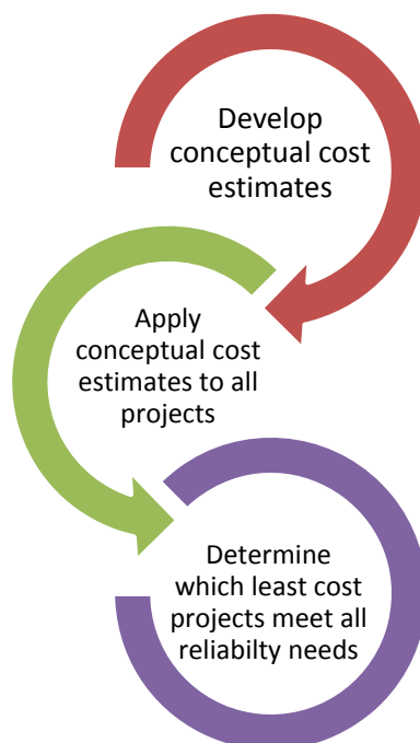
Figure 4.2: Project Selection
