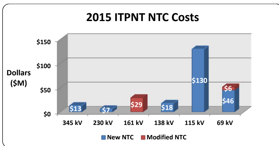
Figure 5.5: 2015 ITPNT NTC Costs by Voltage Class
